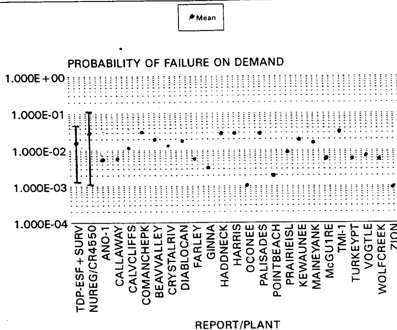
PWR AFW SYSTEM TDPs
