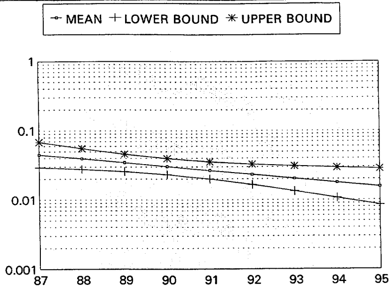
BWR HPCI SYSTEM TDP PROBABILITY OF FAILURE ON DEMAND YEARLY TREND - 1987-1995 FIGURE 3
