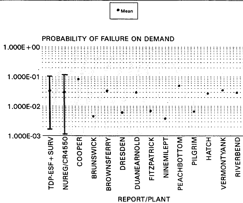
BWR HPCI SYSTEM TDP PROBABILITY OF FAILURE ON DEMAND COMPARISON WITH VALUES USED IN IPEs FIGURE 6
