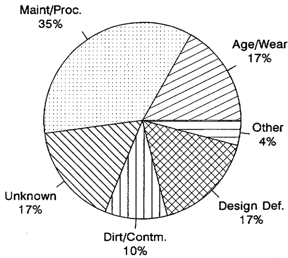
BWR HPCI SYSTEM TDP FAILURE CAUSES FIGURE 13
