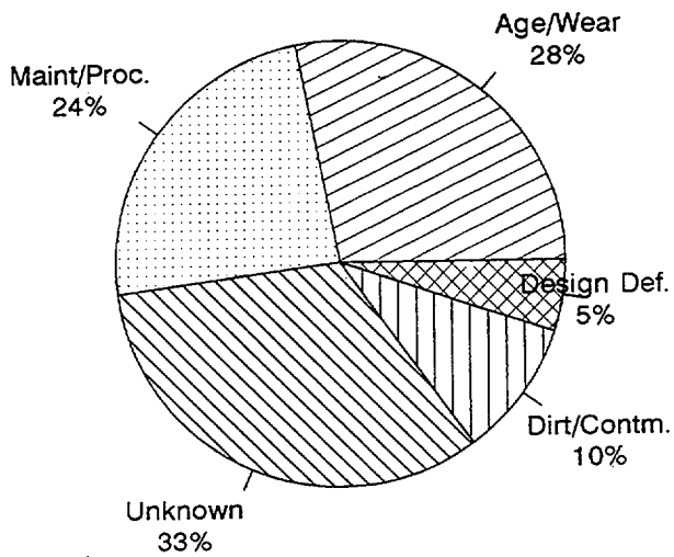
BWR RCIC SYSTEM TDP FAILURE CAUSES FIGURE 12
