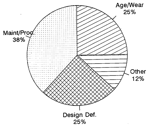
BWR RCIC SYSTEM TDP FAILURE CAUSES FIGURE 12
