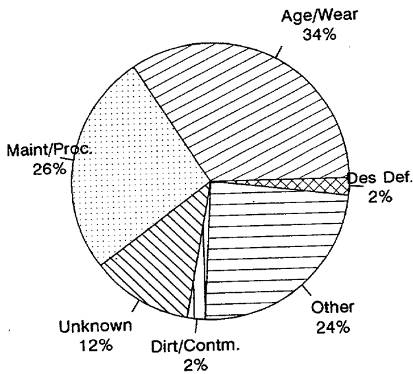
PWR AFW SYSTEM TDP FAILURE CAUSES FIGURE 11
