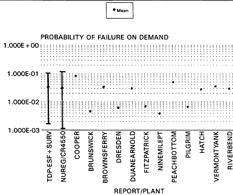
FIGURE ES-3 BWR HPCI SYSTEM TDP PROBABILITY OF FAILURE ON DEMAND COMPARISON WITH VALUES USED IN IPEs
