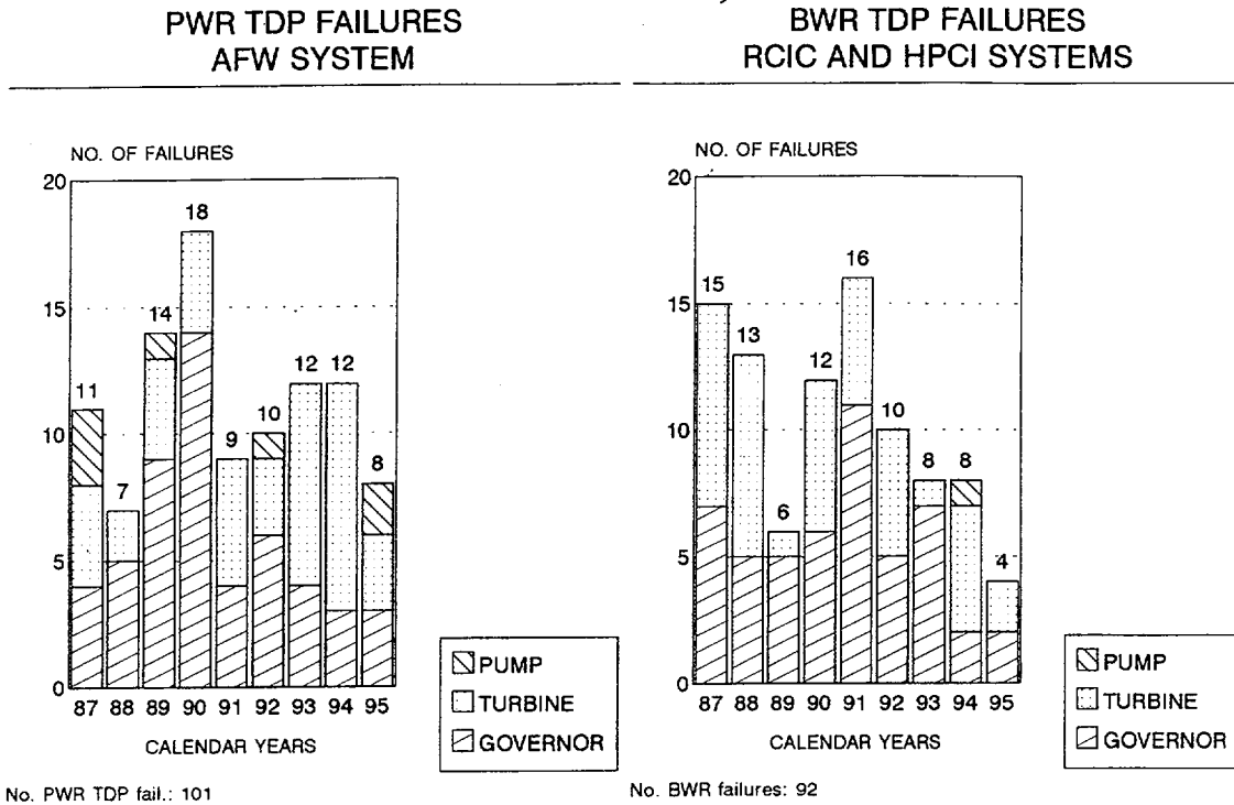
FIGURE ES-4 TDP FAILURE TRENDS
