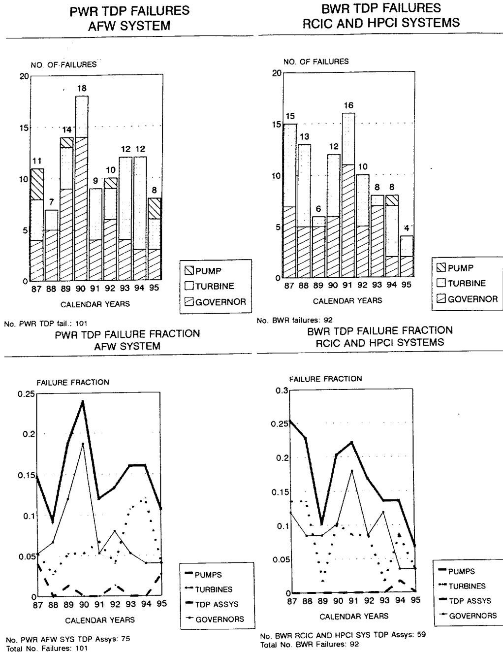
PWR AND BWR TDP FAILURE TRENDS FIGURE 7
