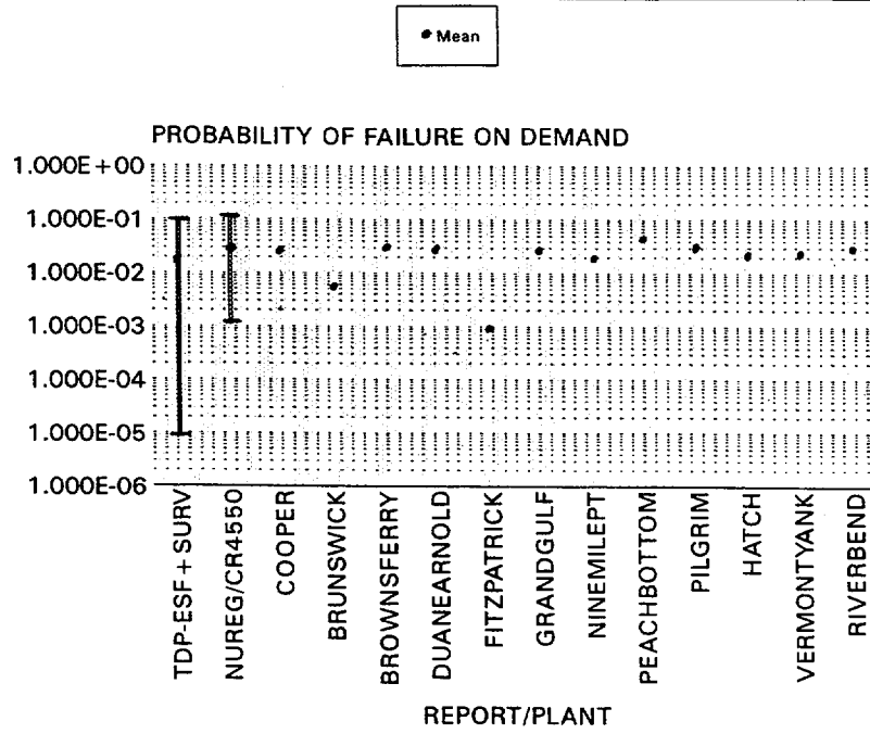
FIGURE ES-2 BWR RCIC SYSTEM TDP PROBABILITY OF FAILURE ON DEMAND COMPARISON WITH VALUES USED IN IPEs
